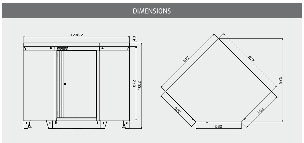
ART. NO. 47505 MSS 34" CORNER CLOSET NO TOP BLADE ART. NO. 4731414 MSS 34" CORNER CLOSET WOODEN TOP BLADE ART. NO. 4731714 34" CORNER CLOSET STAINLESS STEEL TOP BLADE
