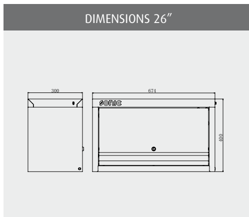
ART. NO. 47276 26" CUPBOARD L674 X D300 X H400MM ART. NO. 47292 34" CUPBOARD L845 X D300 X H400MM
