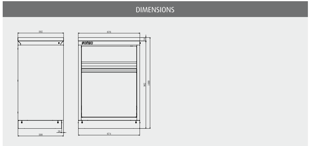
ART. NO. 47431 26" TRASH CAN CLOSET NO TOP BLADE ART. NO. 4731316 26" TRASH CAN CLOSET WOODEN TOP BLADE ART. NO. 4731616 26" TRASH CAN CLOSET STAINLESS STEEL TOP BLADE
