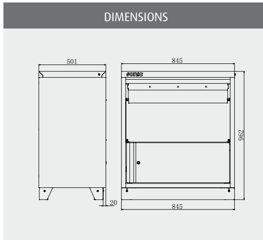
ART. NO. 47600 34" CLOSET FOR REELS NO TOP BLADE ART. NO. 4731416 34" CLOSET FOR REELS WOODEN TOP BLADE ART. NO. 4731618 34" CLOSET FOR REELS STAINLESS STEEL TOP BLADE
