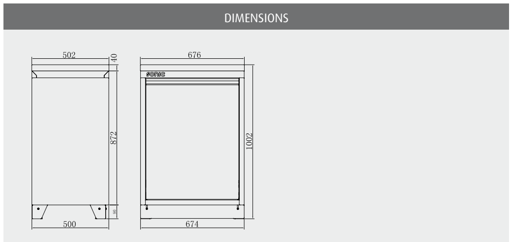
ART. NO. 47450 26" RECYCLE BIN ART. NO. 4731312 26" RECYCLE BIN WOODEN TOP BLADE ART. NO. 4731612 26" RECYCLE BIN STAINLESS STEEL TOP BLADE
