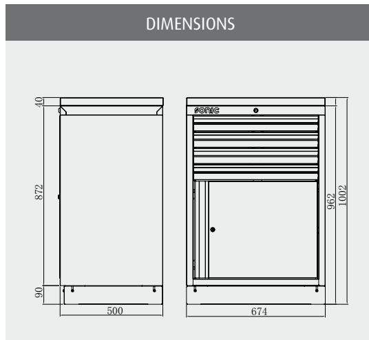
ART. NO. 47308 26" CABINET WITH DOOR NO TOP BLADE ART. NO. 4731310 26" CABINET WITH DOOR WOODEN TOP BLADE ART. NO. 4731610 26" CABINET WITH DOOR STAINLESS STEEL T. B.
