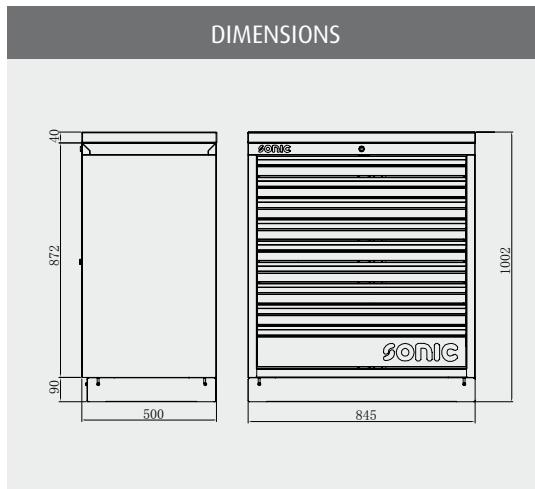
ART. NO. 4731707 34" CABINET STAINLESS STEEL TOP BLADE
