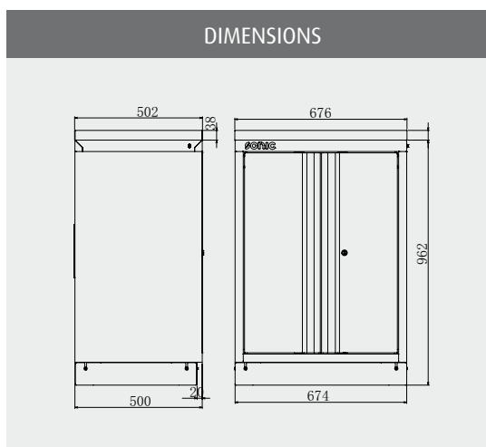
ART. NO. 47432 26" CLOSET WITH SINK NO TOP ART. NO. 4731317 26" CLOSET WITH SINK WOODEN ART. NO. 4731617 26" CLOSET WITH SINK STAINLESS STEEL T. B.
