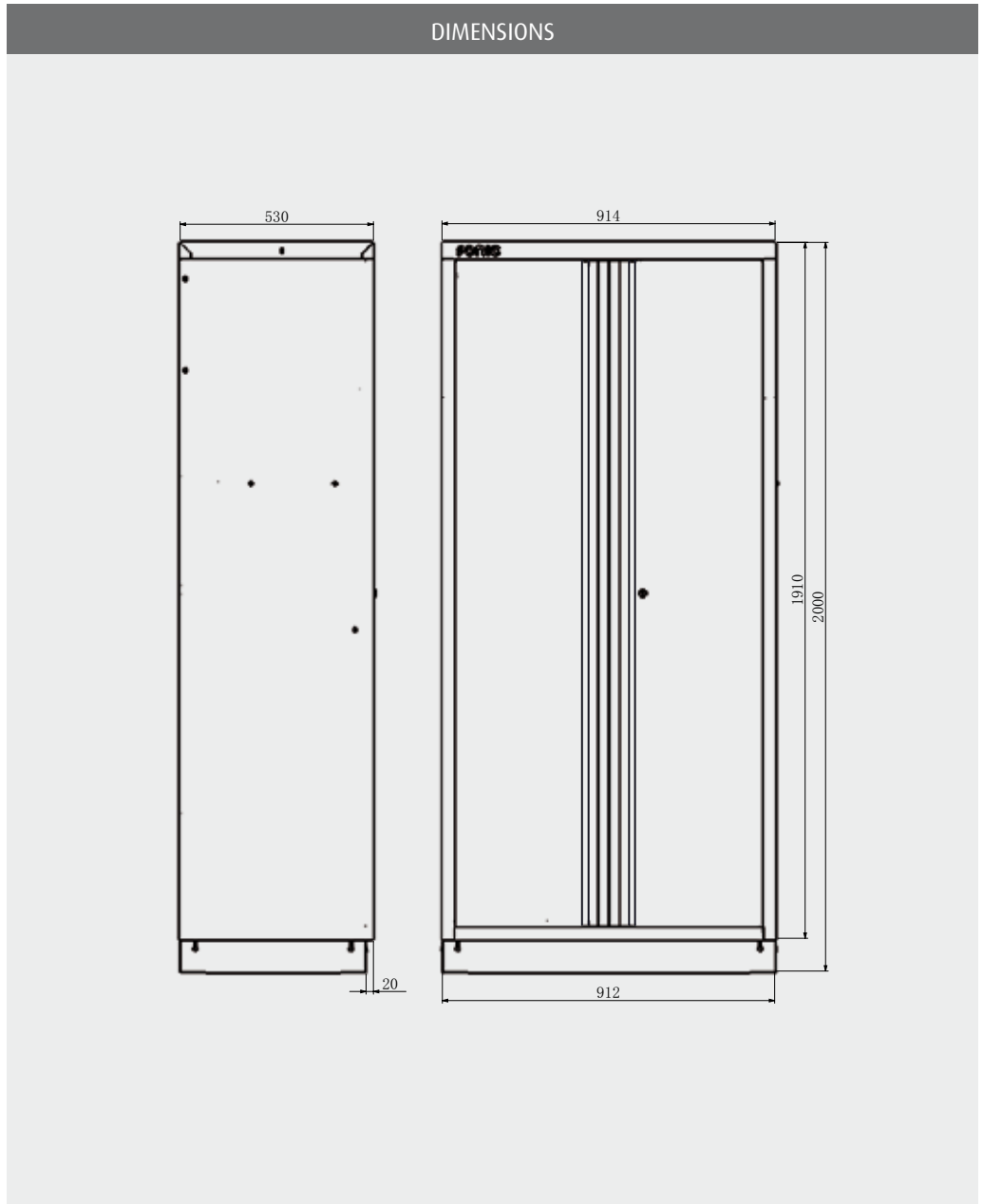
ART. NO. 47433 36" DOUBLE DOOR LOCKER THE LOCKER CONTAINS 4 SHELVES MEASUREMENTS: L910 X D530 X H2000MM
