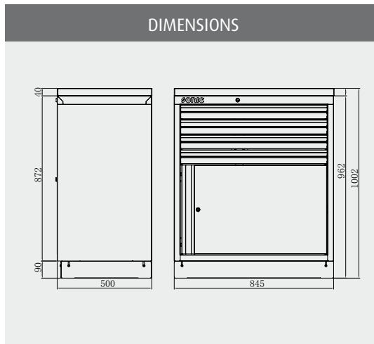
ART. NO. 47379 26" CLOSET NO TOP BLADE ART. NO. 4731410 34" CABINET WITH DOOR WOODEN TOP BLADE ART. NO. 4731710 34" CABINET WITH DOOR STAINLESS STEEL T. B.
