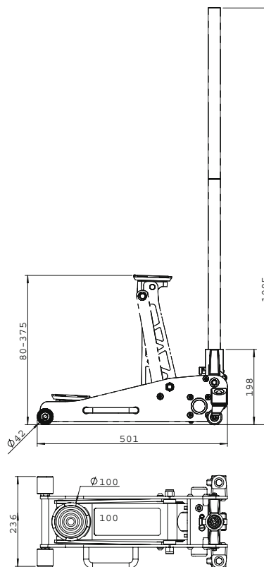
ART. NO. 4800203 INCL. EXTRA RUBBER PAD 95MM
