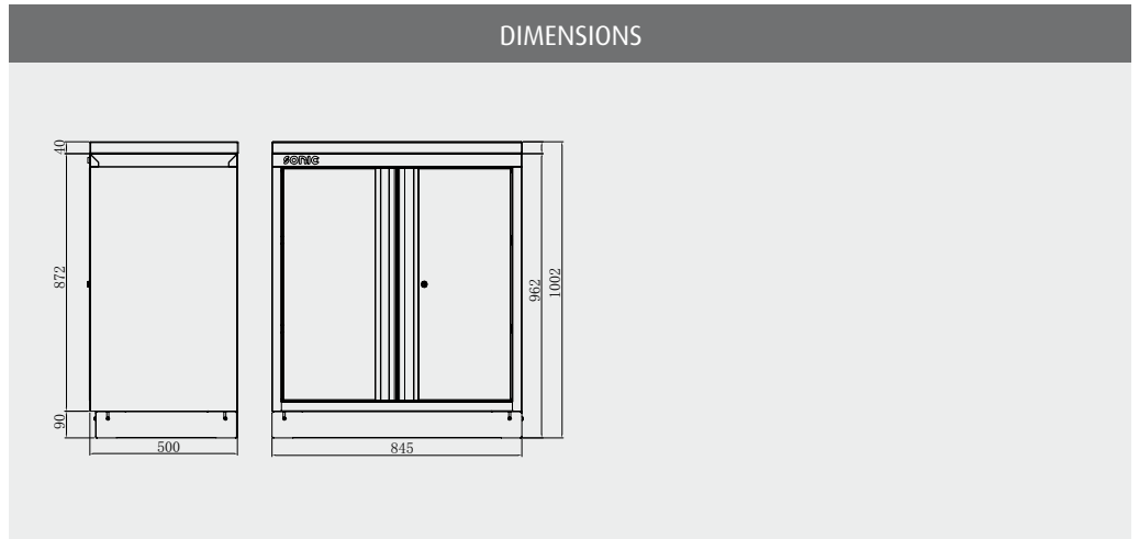
ART. NO. 47302 34" CLOSET NO TOP BLADE ART. NO. 4731408 34" CLOSET WOODEN TOP BLADE ART. NO. 4731708 34" CLOSET STAINLESS STEEL TOP BLADE
