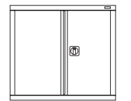
GSC-9150 W 1000mm H 900mm D 550mm
