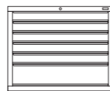
GDU-8150 W 1000mm H 800mm D 550mm
