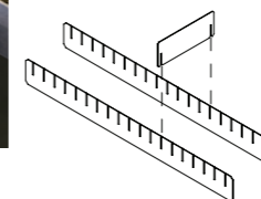
GDD-0500 Drawer divider set for a drawer within a 500mm wide unit. (4 strips, 8 slats)
